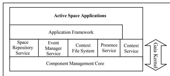
Figure 3. Gaia Architecture
