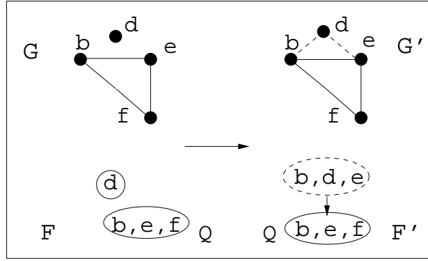
Figure 8. Computing increment of model description length.
