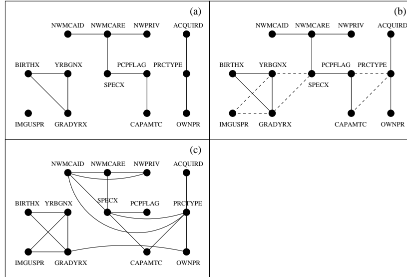
Figure 12. Learned models as DMNs.
