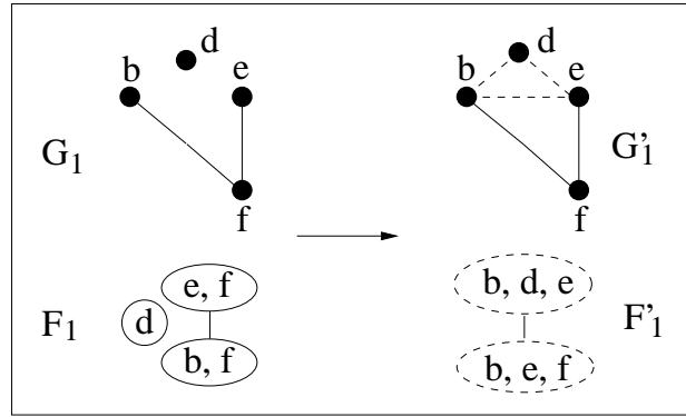
Figure 9. Computing increment of model description length.
