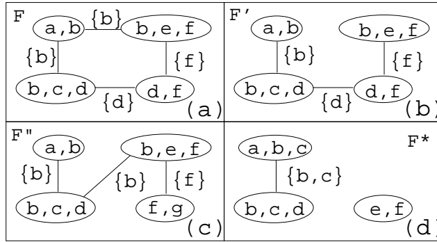
Figure 2. Examples of cluster graphs.
