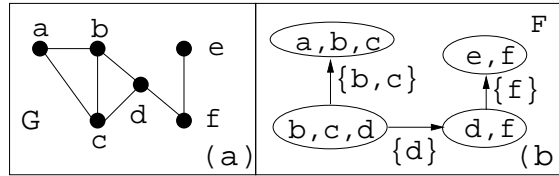
Figure 3. (a) A chordal graph G . (b) a corresponding JF F of G .
