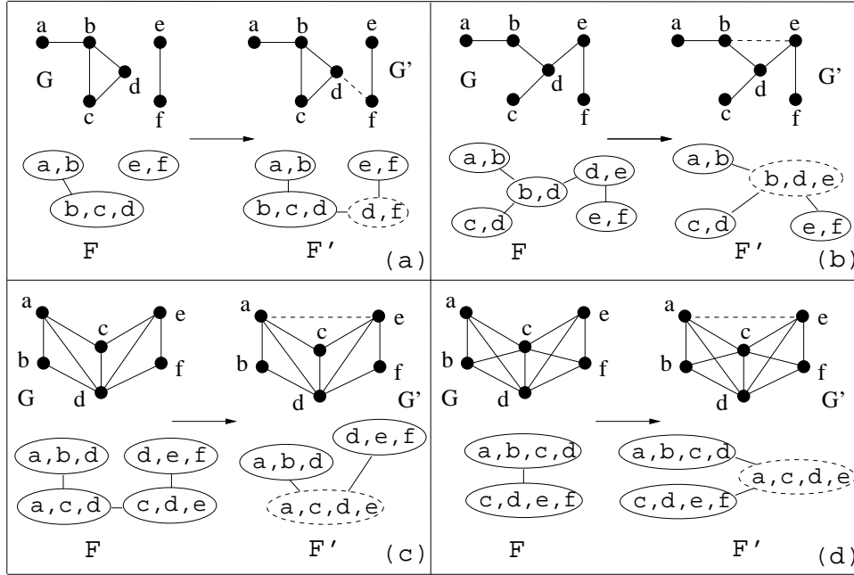
Figure 5. Adding a single link to current graphical structure.
