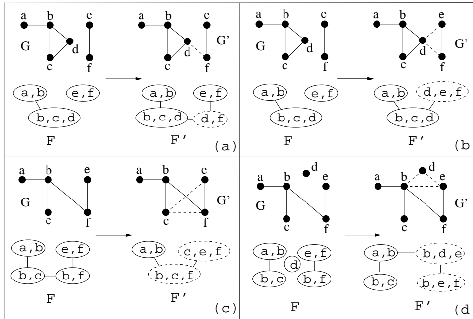
Figure 7. Illustration of crux
