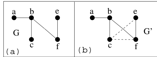
Figure 4. Adding multiple links to current graphical structure. (a) Current chordal graph. (b) Supergraph with two links (dashed) added.
