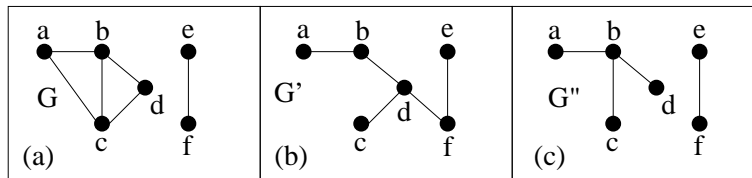
Figure 1. Examples of graphs.
