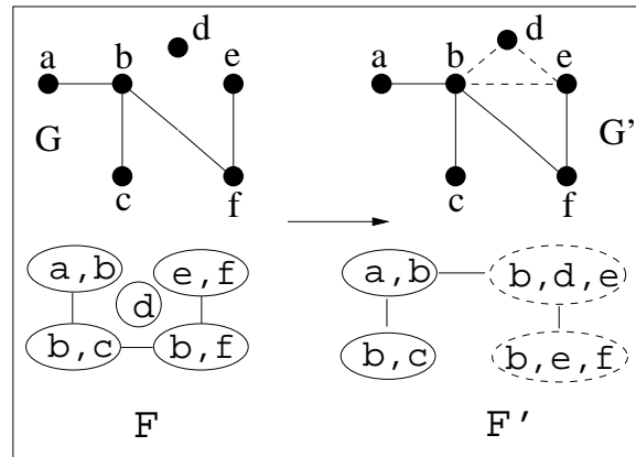
Figure 6. Adding multiple links.
