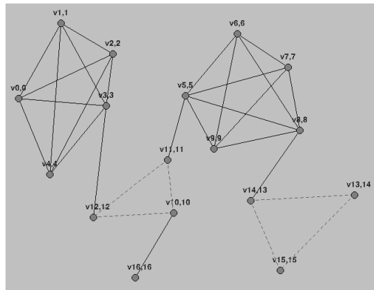
Figure 11. DMN model learned from Bigsma17v domain.
